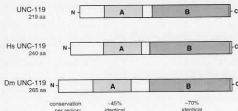
FIGURE 2 Comparison of C. elegans UNC-119, human HsUNC-119 and Drosophila DmUNC-119. (A) Amino acid alignment. Identities present in at least two of the three genes are shown as white text in black boxes, and conserved residues are shaded gray. A single line above the alignment indicates the extent of region A, while a double line shows region B. (B) Schematic alignment of the three homologs showing the two regions A and B, and the percentage identities and conserved changes (similarities) with HsUNC-119.
