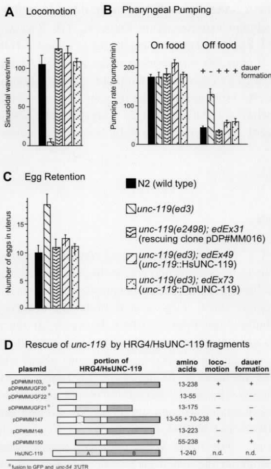
FIGURE 5 Ability of HRG4 and DmUNC-119 transgenes to rescue the C. elegans unc-119 mutant phenotype. (A–C) Rescue of unc-119 behavioral defects by HRG4/HsUNC-119 and DmUNC-119 transgenes. At least ten animals were scored for each trait. Data collection for panels (A–C) is described in Maduro and Pilgrim (1995). Lines above data bars denote standard error of the mean (SEM). (A) Locomotion measured in liquid (M9 buffer). (B) Pharyngeal pumping. ‘+’ denotes ability to form dauer larvae, and ‘-’ denotes a dauer formation defect. (C) Retention of eggs in adult hermaphrodites in the presence of food. (D) Rescue of locomotory and dauer formation defects by truncated HRG4 transgenes. Data collection is described in the text. The structure of the predicted full-length HRG4 protein is shown at the bottom for comparison; conserved regions A and B are shaded. ‘amino acids’ indicates the amino acids of HRG4 present in each transgene. Plasmids pDP#MM103, 147, 148 and 150 were injected into unc-119(e2498) , the GFP fusions pUGF20–22 were injected into unc-119(ed3) , and pDP#MM155 was injected into unc-119(ed3); him-8(e1489) . Plasmids pDP#MM147–155 were coinjected with pRF4 ( rol-6 ) as transgenic markers.
