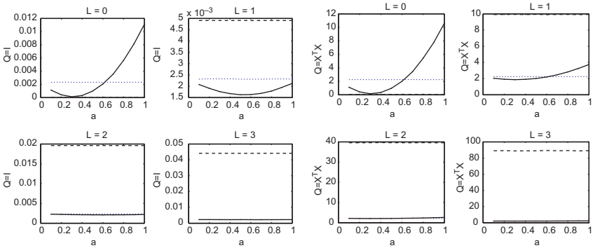
Fig. 8. Risk( \beta(y, X) ) = \mathbb{E}[(\beta(y, X) - \beta)'Q(\beta(y, X) - \beta)] as Function of a . Left Panel: Q = I (MSE), Right Panel: Q = X'X . The Data-Generating Singular Values are Linearly Decreasing from 5 to 1. Other Parameters are Set to K_1 = 1 , \sigma = 3 . The Connected Dots' Line Shows the Performance of the Stein-like Estimator. For Comparison, the Performance of the Standard OLS Estimator is Shown in Dots. The Performance of the Principal Components Estimator is Plotted with Dashes.
