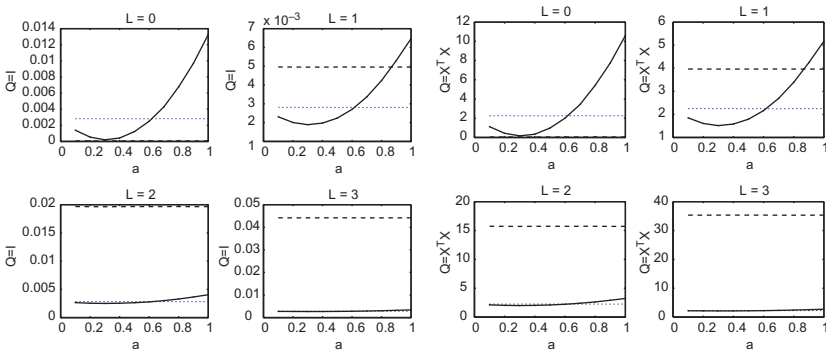
Fig. 7. Risk( \beta(y, X) = \mathbb{E}[(\beta(y, X) - \beta)'Q(\beta(y, X) - \beta)] ) as Function of a . Left Panel: Q = I (MSE), Right Panel: Q = X'X . The Data-Generating Singular Values are Constant and Equal to Two. Other Parameters are Set to K_1 = 1, \sigma = 3 . The Connected Dots' Line Shows the Performance of the Stein-like Estimator. For Comparison, the Performance of the Standard OLS Estimator is Shown in Dots. The Performance of the Principal Components Estimator is Plotted with Dashes.
