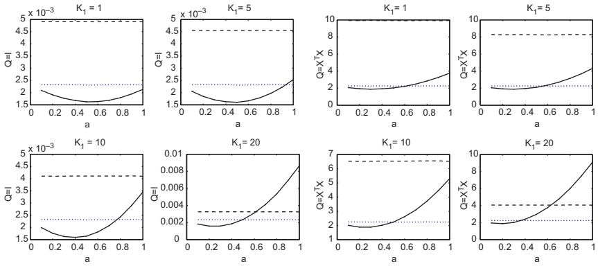
Fig. 2. \text{Risk}(\beta(y, X)) = \mathbb{E}[(\beta(y, X) - \beta)'Q(\beta(y, X) - \beta)] as Function of a . Left Panel: Q = I (MSE), Right Panel: Q = X'X . The Data-Generating Singular Values are Linearly decreasing from 5 to 1. Other Parameters are Set to L = 1 , \sigma = 3 . The Connected Dots' Line Shows the Performance of the Stein-like Estimator. For Comparison, the Performance of the Standard OLS Estimator is shown in Dots. The Performance of the Principal Components Estimator is Plotted with Dashes.
