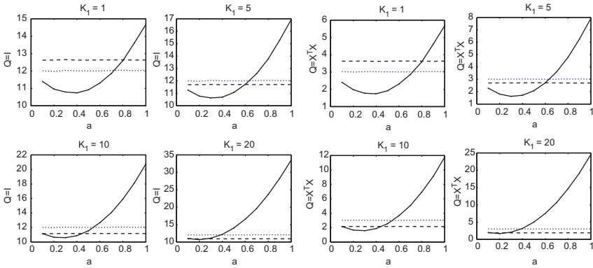
Fig. 10. Left Panel: MSFE(\beta(y, X)) = \mathbb{E}[(\hat{y} - y)'(\hat{y} - y)] , Where \hat{y} is a T_2 -Vector of Forecasts of y , as Function of a . Right Panel: Risk(\beta, \beta(y, X), X'X) = \mathbb{E}[(\beta(y, X) - \beta)'X'X(\beta(y, X) - \beta)] for the T_2 -Period Forecast Sample. The Data-Generating Eigenvalues are Exponentially Decreasing from 5 to 1 at a Rate of 0.10. Other Parameters are Set to L = 1, \sigma = 3 . The Connected Dots' Line Shows the Performance of the Stein-like Estimator. For Comparison, the Performance of the Standard OLS Estimator is Shown in Dots. The Performance of the Principal Components Estimator is Plotted with Dashes.
