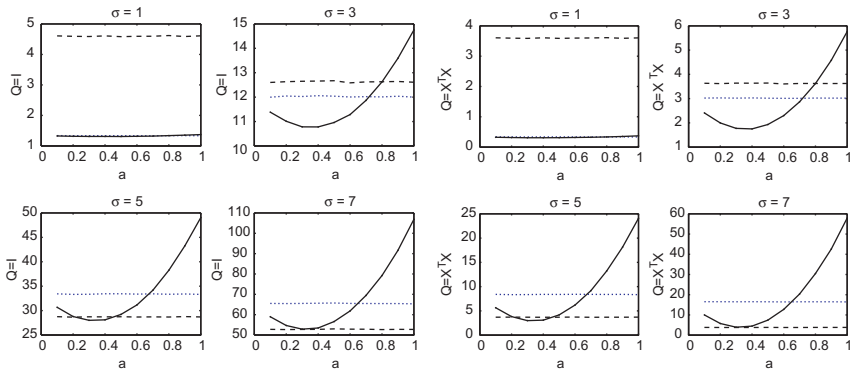
Fig. 12. Left Panel: MSFE(\beta(y, X)) = \mathbb{E}[(\hat{y} - y)'(\hat{y} - y)] , Where \hat{y} is a T_2 -Vector of Forecasts of y , as Function of a . Right Panel: Risk(\beta, \beta(y, X), X'X) = \mathbb{E}[(\beta(y, X) - \beta)'X'X(\beta(y, X) - \beta)] for the T_2 -Period Forecast Sample. The Data-Generating Eigenvalues are Exponentially Decreasing from 5 to 1 at a Rate of 0.10. Other Parameters are Set to K_1 = 1, L = 1 . The Connected Dots' Line Shows the Performance of the Stein-like Estimator. For Comparison, the Performance of the Standard OLS Estimator is Shown in Dots. The Performance of the Principal Components Estimator is Plotted with Dashes.
