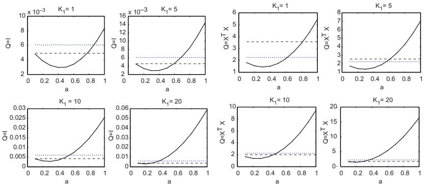
Fig. 3. \text{Risk}(\beta(y, X)) = \mathbb{E}[(\beta(y, X) - \beta)'Q(\beta(y, X) - \beta)] as Function of a . Left Panel: Q = I (MSE), Right Panel: Q = X'X . The Data-Generating Singular Values are Exponentially Decreasing from 5 to 1 at a Rate of 0.10. Other Parameters are Set to L = 1 , \sigma = 3 . The Connected Dots' Line Shows the Performance of the Stein-like Estimator. For Comparison, the Performance of the Standard OLS Estimator is shown in Dots. The Performance of the Principal Components Estimator is Plotted with Dashes.
