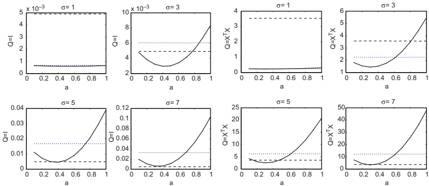
Fig. 6. Risk( \beta(y, X) = \mathbb{E}[(\beta(y, X) - \beta)'Q(\beta(y, X) - \beta)] ) as Function of a . Left Panel: Q = I (MSE), Right Panel: Q = X'X . The Data-Generating Singular Values are Exponentially Decreasing from 5 to 1 at a Rate of 0.10. Other Parameters are Set to L = 1, K_1 = 1 . The Connected Dots' Line Shows the Performance of the Stein-like Estimator. For Comparison, the Performance of the Standard OLS Estimator is Shown in Dots. The Performance of the Principal Components Estimator is Plotted with Dashes.
