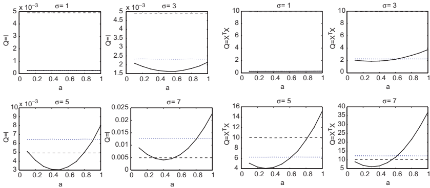
Fig. 5. Risk( \beta(y, X) = \mathbb{E}[(\beta(y, X) - \beta)'Q(\beta(y, X) - \beta)] ) as Function of a . Left Panel: Q = I (MSE), Right Panel: Q = X'X . The Data-Generating Singular Values are Linearly Decreasing from 5 to 1. Other Parameters Are Set to L = 1, K_1 = 1 . The Connected Dots' Line Shows the Performance of the Stein-like Estimator. For Comparison, the Performance of the Standard OLS Estimator is Shown in Dots. The Performance of the Principal Components Estimator is Plotted with Dashes.
