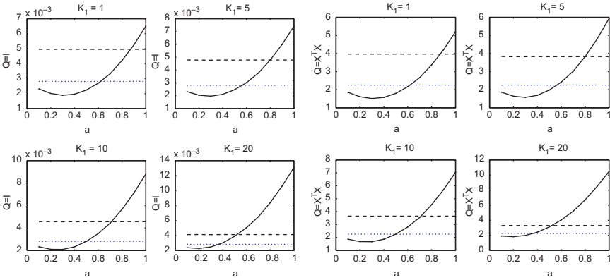
Fig. 1. Risk( \beta(y, X) ) = \mathbb{E}[(\beta(y, X) - \beta)'Q(\beta(y, X) - \beta)] as Function of a . Left Panel: Q = I (MSE), Right Panel: Q = X'X . The Data-Generating Singular Values are Constant and Equal to Two. Other Parameters Are Set to L = 1 , \sigma = 3 . The Connected Dots' Line Shows the Performance of the Stein-like Estimator. For Comparison, the Performance of the Standard OLS Estimator is Shown in Dots. The Performance of the Principal Components Estimator is Plotted with Dashes.
