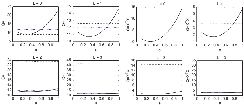
Fig. 14. Left Panel: MSFE(\beta(y, X)) = \mathbb{E}[(\hat{y} - y)'(\hat{y} - y)] , Where \hat{y} Is a T_2 -Vector of Forecasts of y , as Function of a . Right Panel: Risk(\beta, \beta(y, X), X'X) = \mathbb{E}[(\beta(y, X) - \beta)'X'X(\beta(y, X) - \beta)] for the T_2 -Period Forecast Sample. The Data-Generating Eigenvalues are Exponentially Decreasing from 5 to 1 at a Rate of 0.10. Other Parameters are Set to K_1 = 1 , \sigma = 3 . The Connected Dots' Line Shows the Performance of the Stein-like Estimator. For Comparison, the Performance of the Standard OLS Estimator is Shown in Dots. The Performance of the Principal Components Estimator is Plotted with Dashes.
