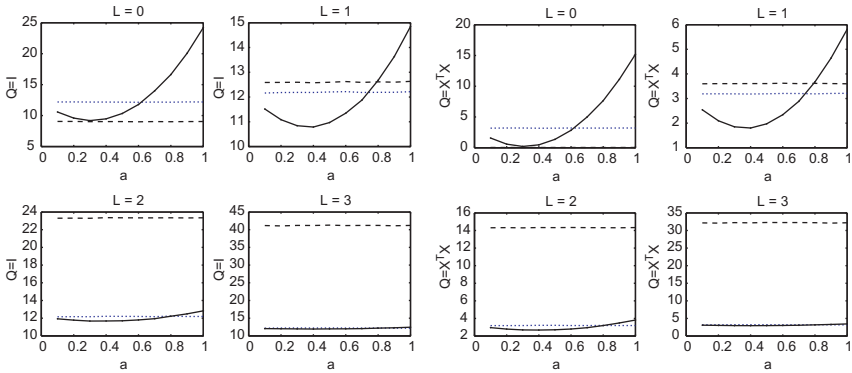
Fig. 15. Left Panel: MSFE(\beta(y, X)) = \mathbb{E}[(\hat{y} - y)'(\hat{y} - y)] , Where \hat{y} is a T_2 -Vector of Forecasts of y , as Function of a . Right Panel: Risk(\beta, \beta(y, X), X'X) = \mathbb{E}[(\beta(y, X) - \beta)'X'X(\beta(y, X) - \beta)] for the T_2 -Period Forecast Sample. The Columns of the Regressor Matrix X are AR(1) Processes. Other Parameters are Set to K_1 = 1, \sigma = 3 . The Connected Dots' Line Shows the Performance of the Stein-like Estimator. For Comparison, the Performance of the Standard OLS Estimator is Shown in Dots. The Performance of the Principal Components Estimator is Plotted with Dashes.
