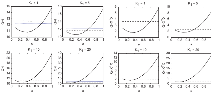
Fig. 11. Left Panel: MSFE(\beta(y, X)) = \mathbb{E}[(\hat{y} - y)'(\hat{y} - y)] , Where \hat{y} is a T_2 -Vector of Forecasts of y , as Function of a . Right Panel: Risk(\beta, \beta(y, X), X'X) = \mathbb{E}[(\beta(y, X) - \beta)'X'X(\beta(y, X) - \beta)] for the T_2 -Period Forecast Sample. The Columns of the Regressor Matrix X are AR(1) Processes. Other Parameters are Set to L = 1, \sigma = 3 . The Connected Dots' Line Shows the Performance of the Stein-like Estimator. For Comparison, the Performance of the Standard OLS Estimator is Shown in Dots. The Performance of the Principal Components Estimator is Plotted with Dashes.
