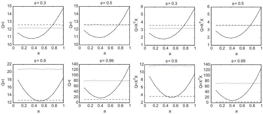
Fig. 13. Left Panel: MSFE(\beta(y, X)) = \mathbb{E}[(\hat{y} - y)'(\hat{y} - y)] , Where \hat{y} is a T_2 -Vector of Forecasts of y , as Function of a . Right Panel: Risk(\beta, \beta(y, X), X'X) = \mathbb{E}[(\beta(y, X) - \beta)'X'X(\beta(y, X) - \beta)] for the T_2 -Period Forecast Sample. The Columns of the Regressor Matrix X are AR(1) Processes. Other Parameters are Set to K_1 = 1 , L = 1 . The Connected Dots' Line Shows the Performance of the Stein-like Estimator. For Comparison, the Performance of the Standard OLS Estimator is Shown in Dots. The Performance of the Principal Components Estimator is Plotted with Dashes.
