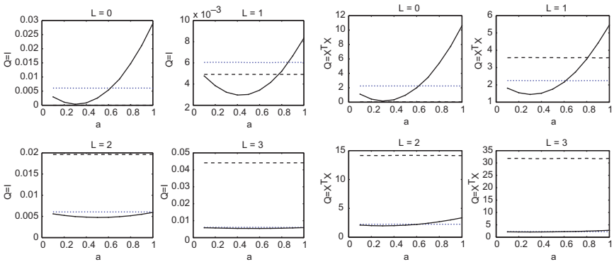
Fig. 9. Risk( \beta(y, X) ) = \mathbb{E}[(\beta(y, X) - \beta)'Q(\beta(y, X) - \beta)] as Function of a . Left Panel: Q = I (MSE), Right Panel: Q = X'X . The Data-Generating Singular Values are Exponentially Decreasing from 5 to 1 at a Rate of 0.10. Other Parameters are Set to K_1 = 1 , \sigma = 3 . The Connected Dots' Line Shows the Performance of the Stein-like Estimator. For Comparison, the Performance of the Standard OLS Estimator is Shown in Dots. The Performance of the Principal Components Estimator is Plotted with Dashes.
