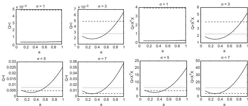
Fig. 4. Risk( \beta(y, X) ) = \mathbb{E}[(\beta(y, X) - \beta)'Q(\beta(y, X) - \beta)] as Function of a . Left Panel: Q = I (MSE), Right Panel: Q = X'X . The Data-Generating Singular Values are Constant and Equal to Two. Other Parameters are Set to L = 1, K_1 = 1 . The Connected Dots' Line Shows the Performance of the Stein-like Estimator. For Comparison, the Performance of the Standard OLS Estimator is Shown in Dots. The Performance of the Principal Components Estimator is Plotted with Dashes.
