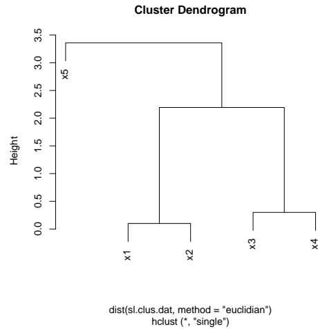
Figure 7.8: Tree of single linkage cluster analysis.
