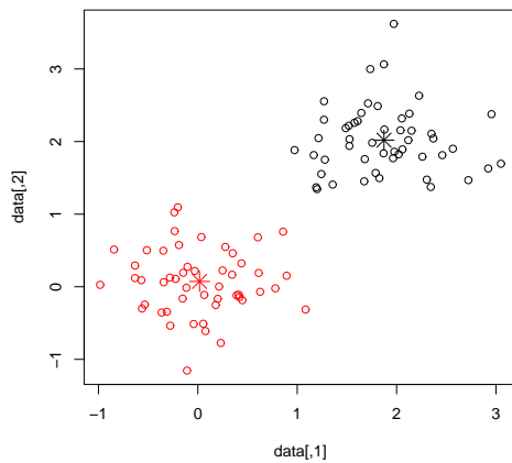
Figure 7.7: K-means cluster analysis.
