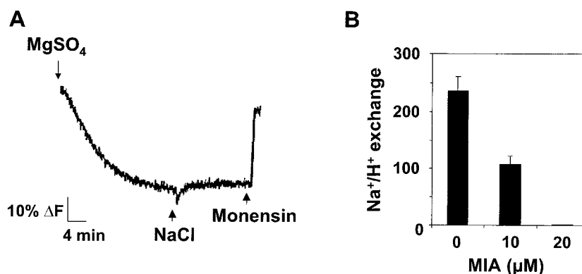
FIG. 3. Tonoplast \text{Na}^+/\text{H}^+ exchange in wild-type Arabidopsis cells is sensitive to methyl-isobutyl amiloride. Tonoplast vesicles were isolated from the cell cultures of wild-type Arabidopsis . Reaction mixes and assay conditions were as described in the legend to Fig. 2. A , a more potent form of amiloride, MIA (20 \mu\text{M} ) was added before \Delta\text{pH} formation was initiated. After the formation of \Delta\text{pH} , NaCl (50 mM) was added to initiate \text{Na}^+/\text{H}^+ exchange. Monensin (150 \mu\text{M} ), was added at the end of the assay to determine if a \Delta\text{pH} was present. B , initial rates of \text{Na}^+/\text{H}^+ exchange as a function of MIA concentration. Data represents means \pm S.E. of the three replicates; units are \Delta\% \text{ F mg}^{-1} \text{ protein min}^{-1} .
