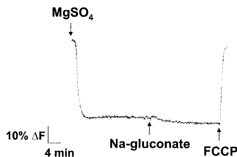
FIG. 4. Tonoplast \text{Na}^+/\text{H}^+ exchange in wild-type Arabidopsis cells is electroneutral. Assays (1 ml) contained 3 \mu\text{M} Oxonol V (Sigma-Aldrich), 0.3 mM \text{PP}_i -BTP, 2 mM \text{MgSO}_4 , 10 mM potassium iminodiacetic acid, 30 mM BTP-Hepes (pH 8.5), 250 mM mannitol, and 50 \mu\text{g} tonoplast protein. Reactions were illuminated at 580 nm and Oxonol V fluorescence was monitored at 650 nm. An inside-acid positive \Delta\psi was formed when tonoplast protein (50 \mu\text{g} ) was added to the reaction mix. Once \Delta\psi reached steady state, sodium gluconate (50 mM) was added to initiate \text{Na}^+/\text{H}^+ exchange. At the end of the experiment, the protonophore carbonyl cyanide p -trifluoromethoxyphenylhydrazone ( FCCP , 5 \mu\text{M} ) was added to determine if a \Delta\psi was present. One representative experiment of three replicates is shown; each replicate experiment was performed using independent membrane preparations.
